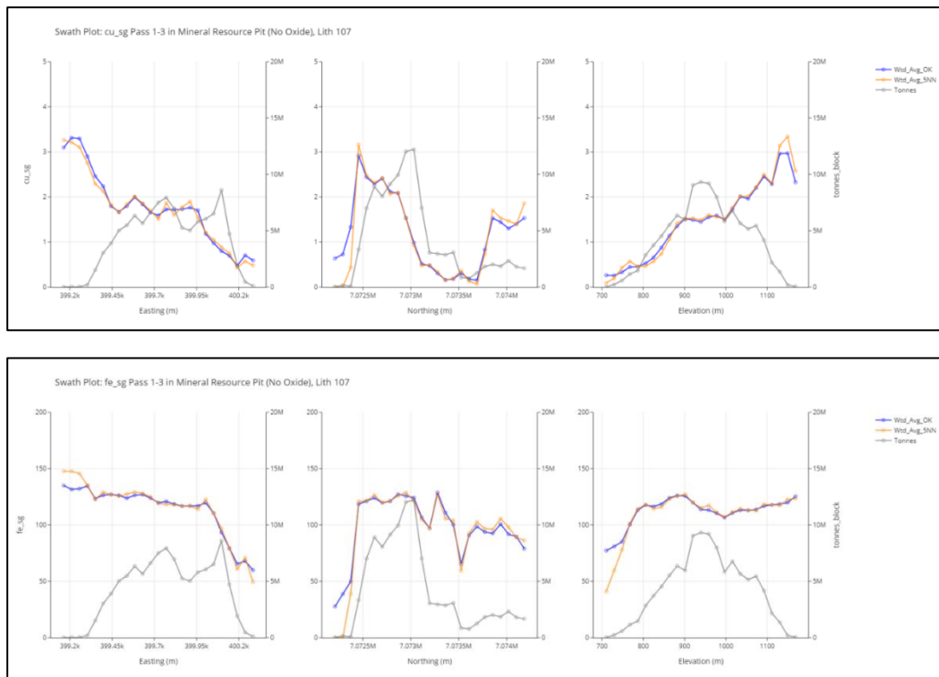
Figure 14-17: Example Swath Plots: SD Cu_SG and Fe_SG, Class 1 and 2 Material
