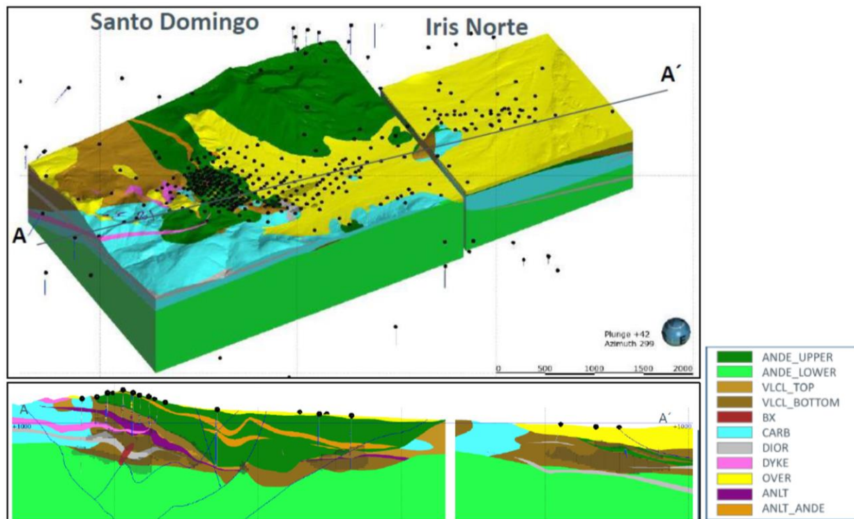
Figure 15-2: Lithological Model
