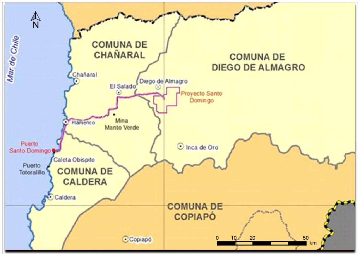
Figure 2-1: Property Location
