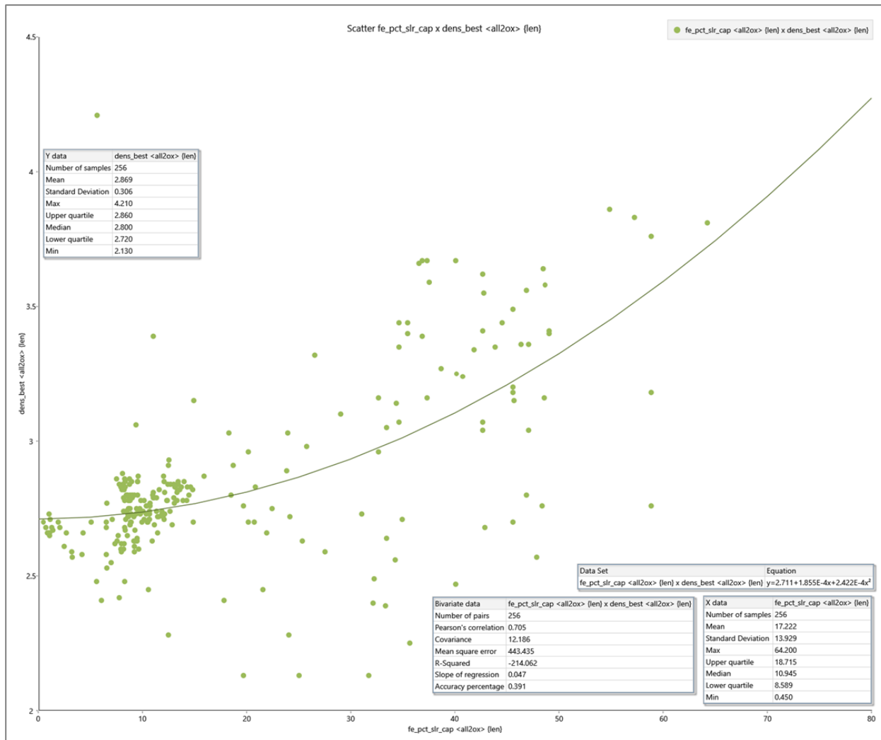
Figure 13-1: Density Regression Curve for Oxide Material: SD + IN
